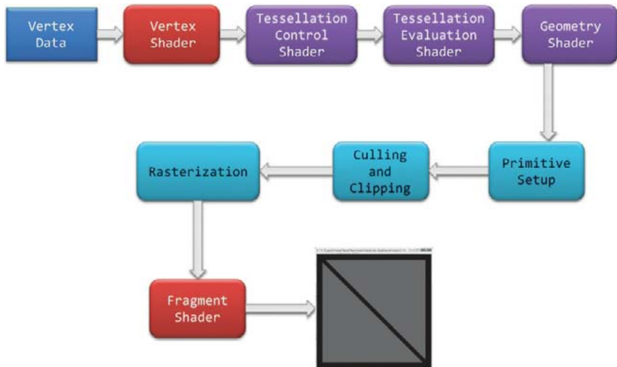
Figure 1.2 OpenGL pipeline
