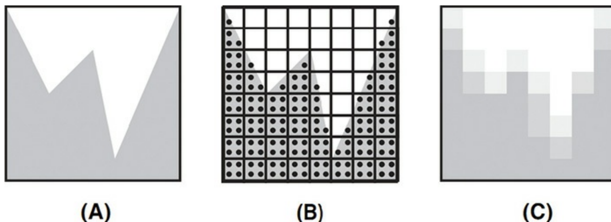
Figure 8.12 Supersampling
