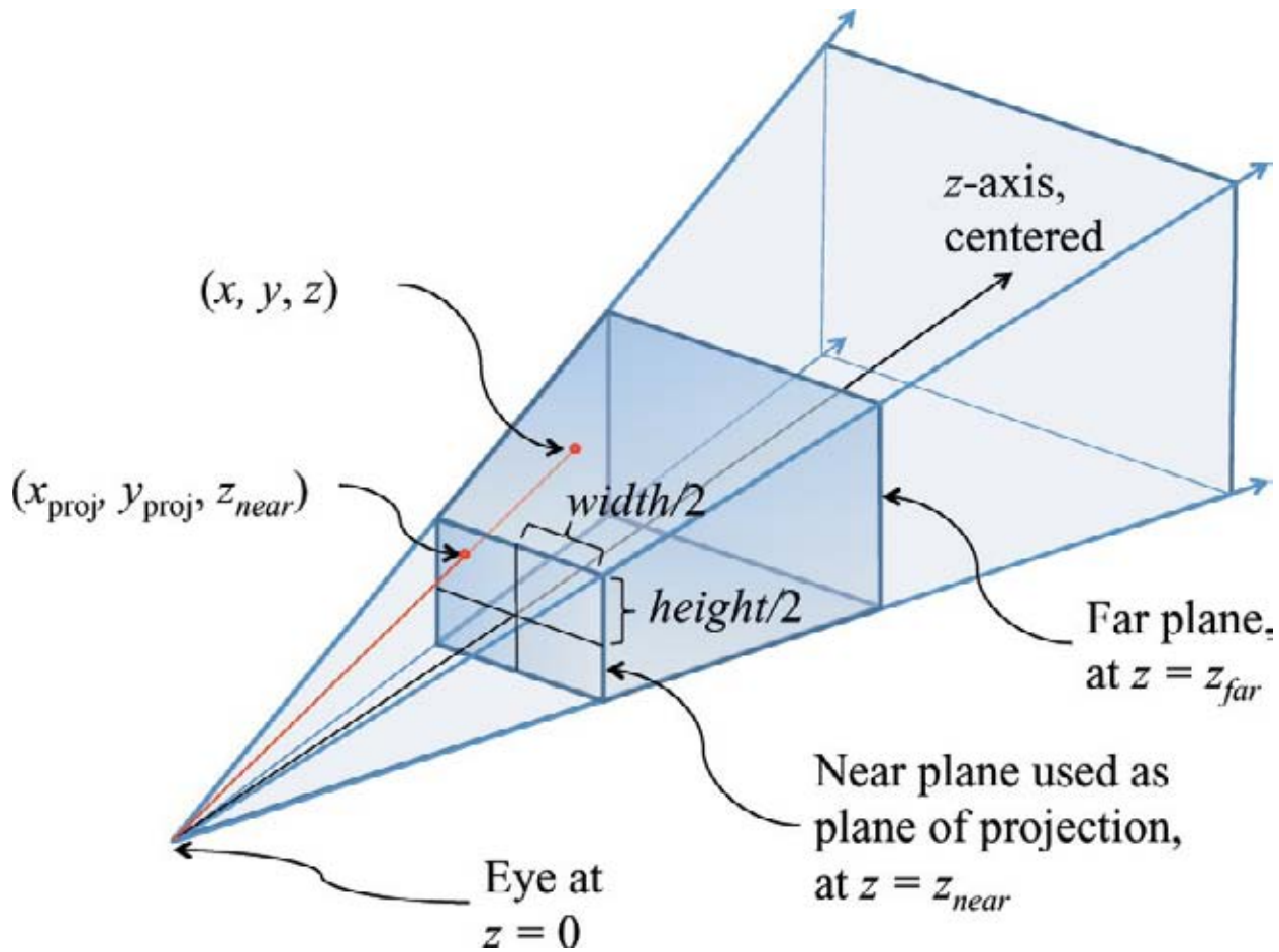
Figure 5.13 Frustum projection
