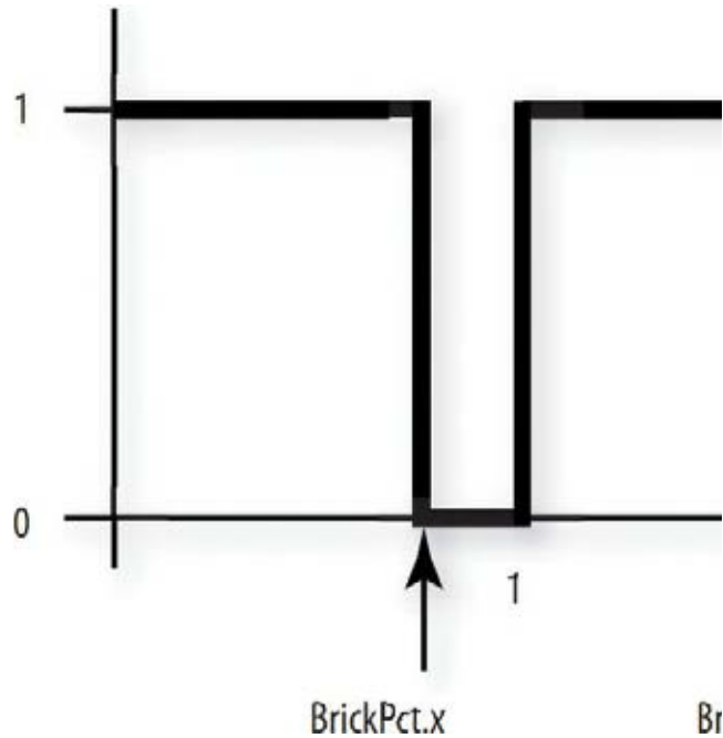
Figure 8.17 The per The periodic step function, or pulse component of the proc
